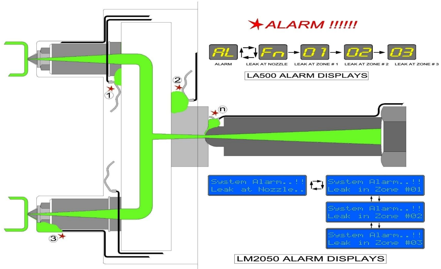
Control/Display Units
